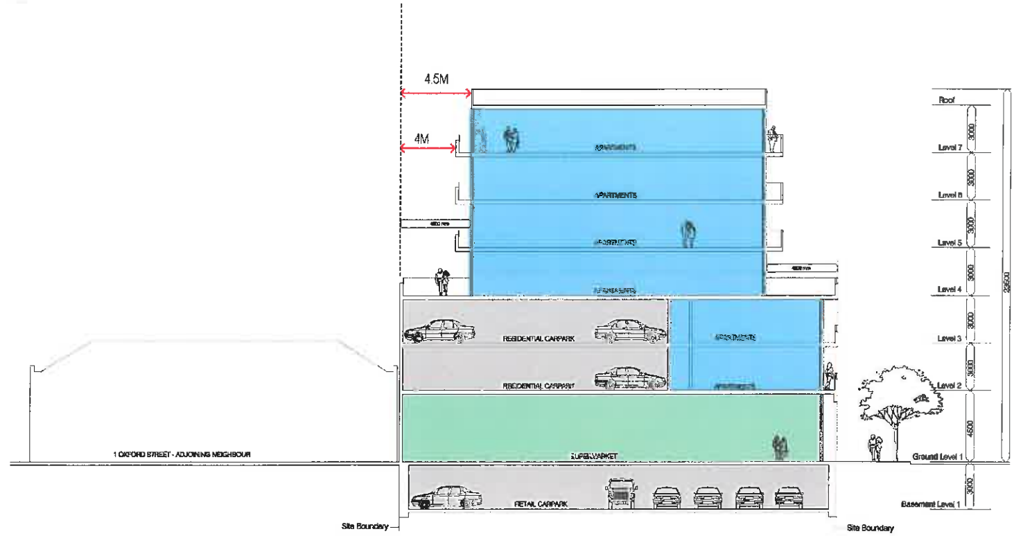
Section BB
